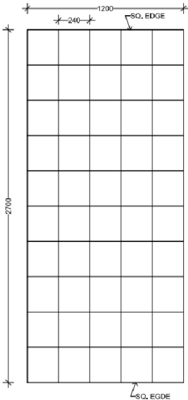
FRONT ELEVATION
