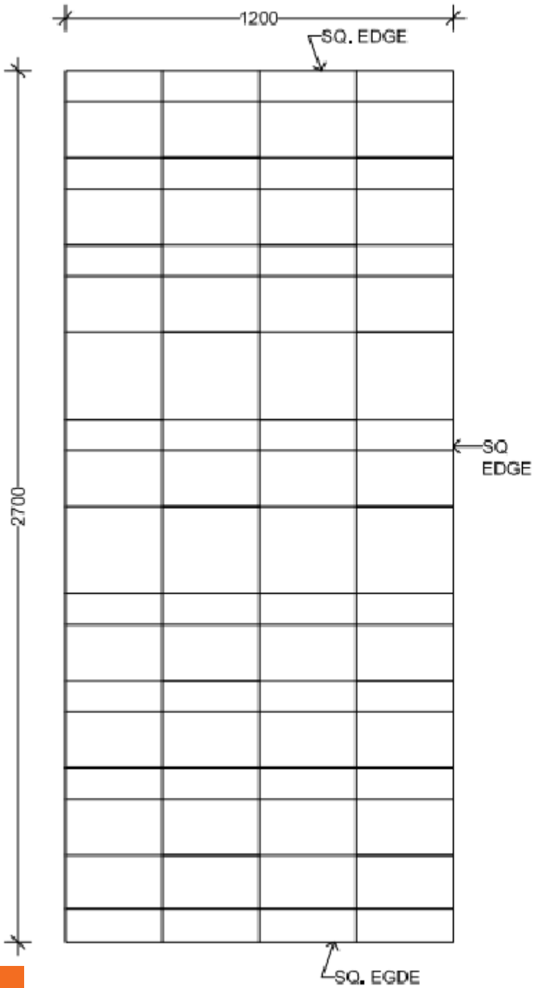
FRONT ELEVATION
