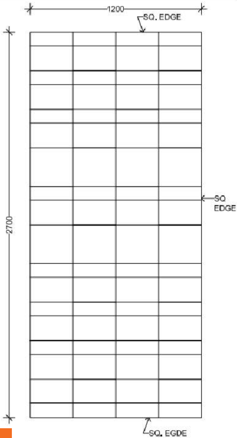
FRONT ELEVATION
