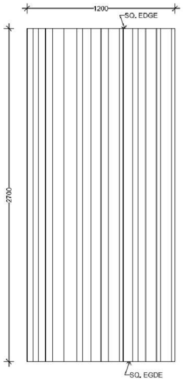
FRONT ELEVATION
