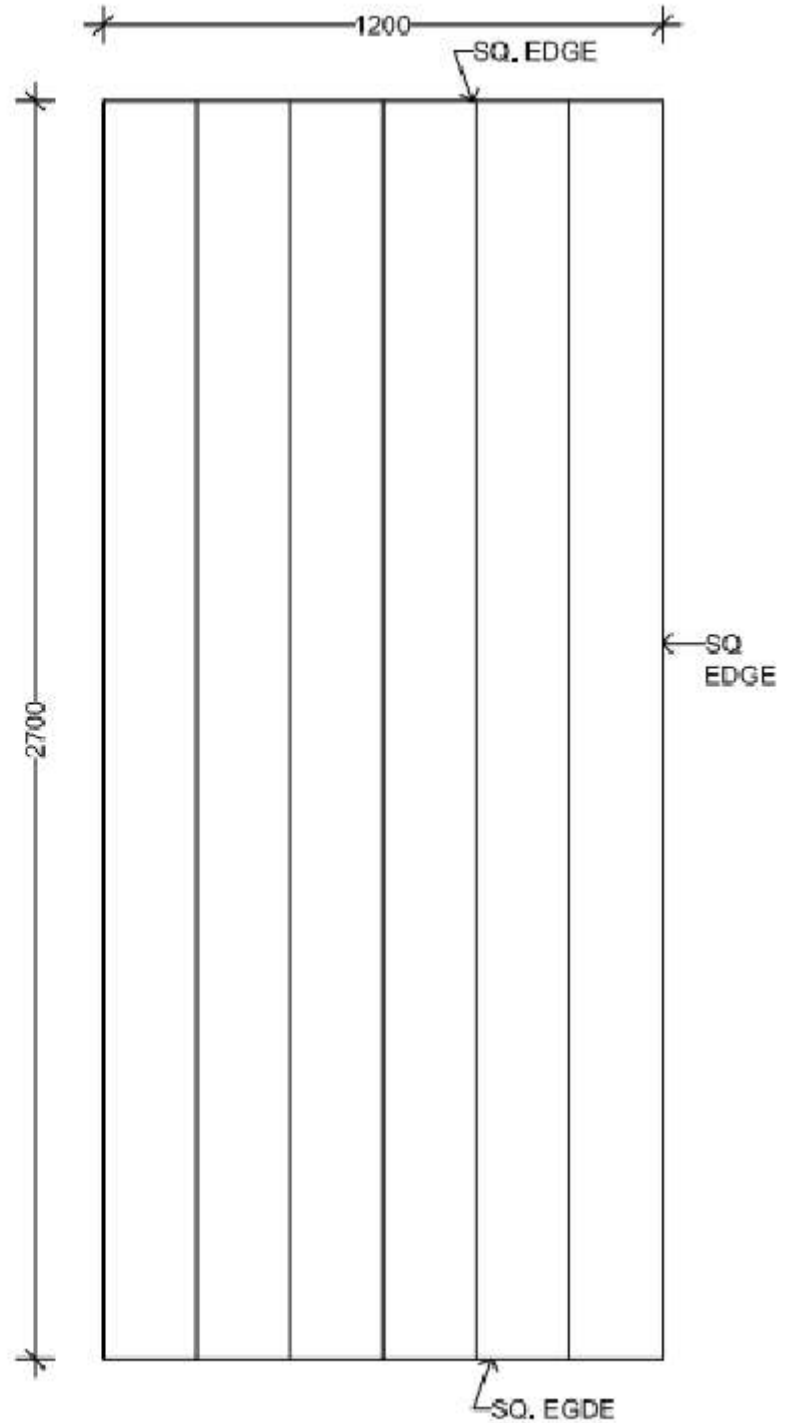
FRONT ELEVATION
