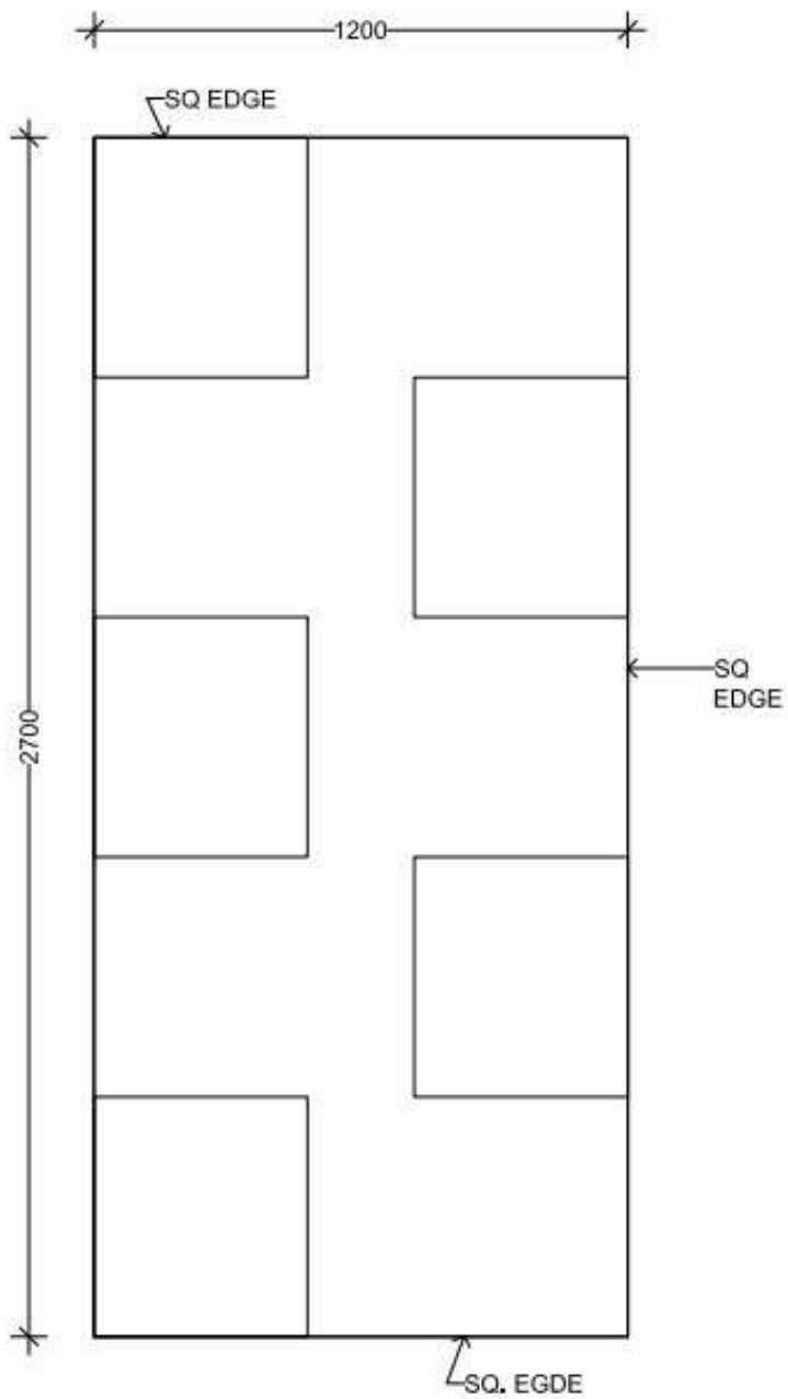
FRONT ELEVATION
